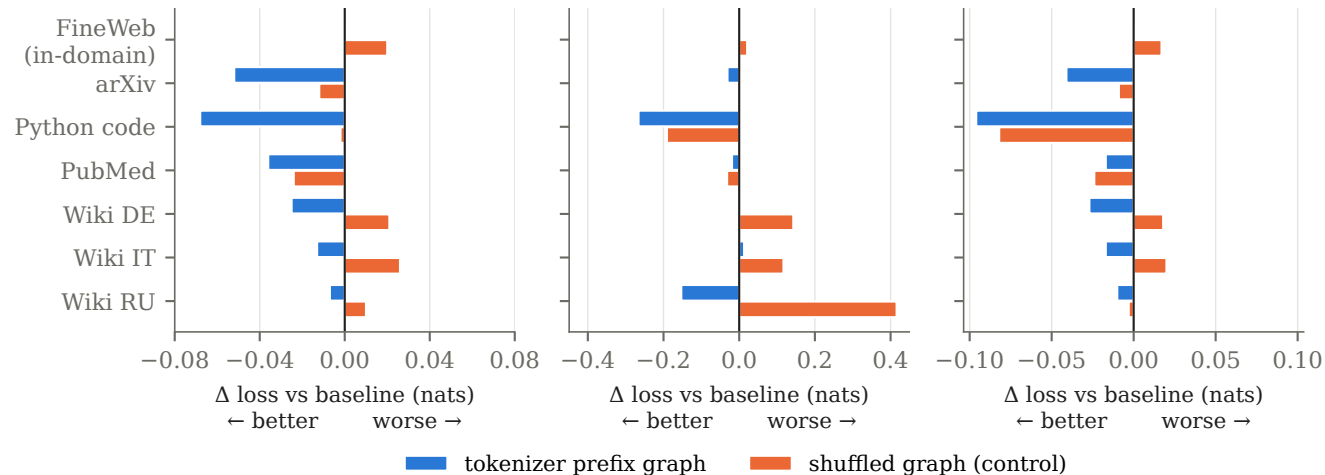
GPT-2 tokenizer, 51M (4 seeds)
