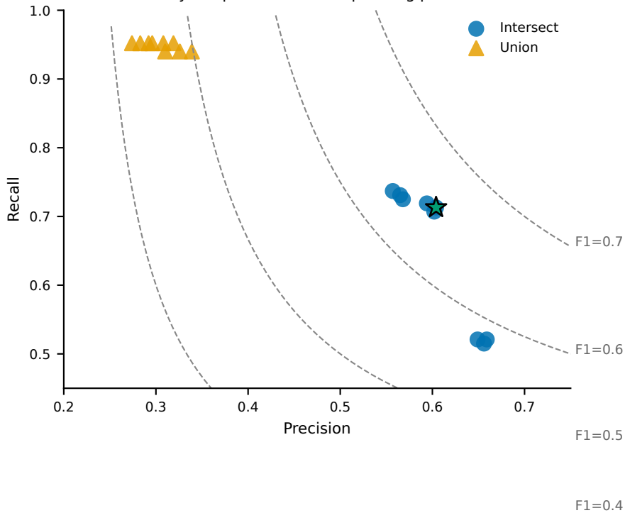
Hybrid precision-recall operating points
