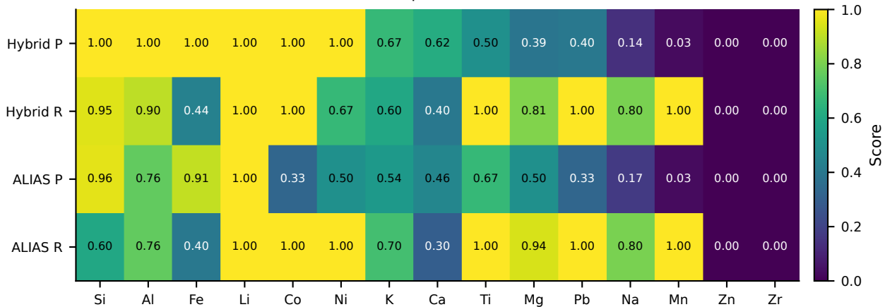
Per-element precision and recall
