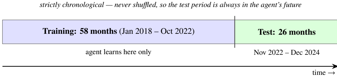
Figure 4.2: Chronological train/test split of the 84 monthly episodes.
