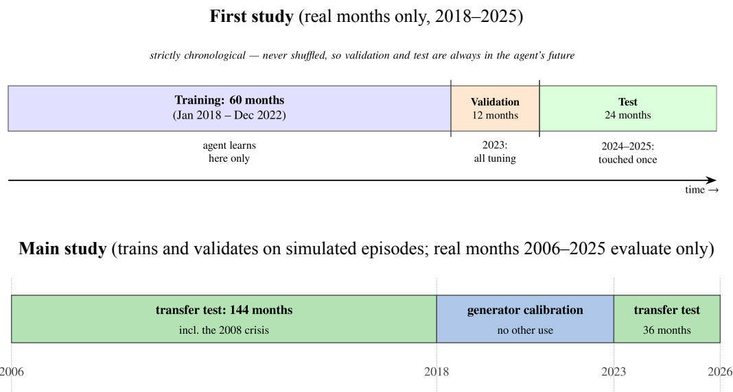
Figure 4.1: How the two studies use the real SPY months. The first study trains, validates, and tests inside 2018–2025 and never touches the earlier years. The main study reads real data only to calibrate the market generator (2018–2022); it trains and validates on simulated episodes, and every other real month — 2006–2017 and 2023–2025, 180 in total — becomes its transfer test.
