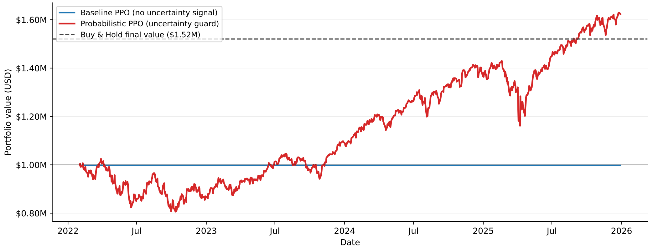
Representative SPY equity curves, 2022-2025 test window
