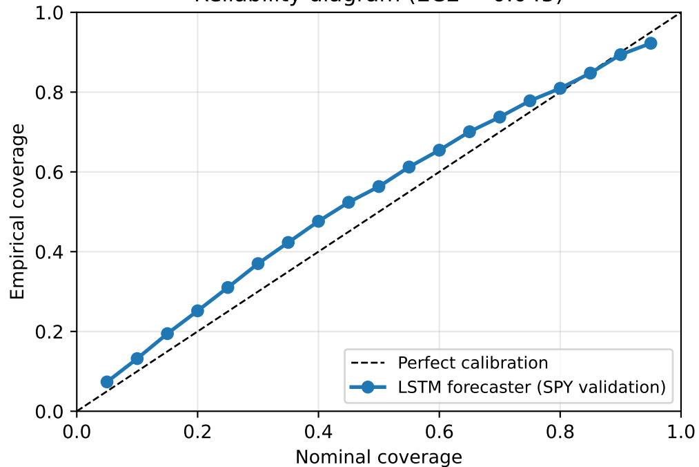
Reliability diagram (ECE = 0.045)
