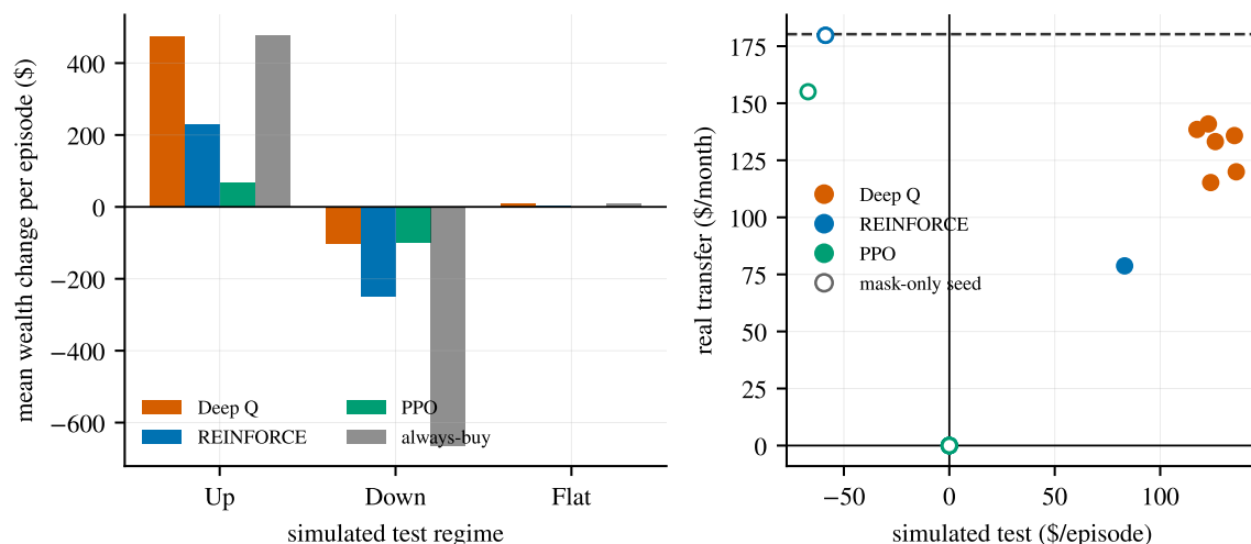
Figure 5.8: Simulated-data study. Left: mean wealth change per episode by test regime for each algorithm and for always-buy. Deep Q-learning keeps almost all of the up-regime profit while cutting the down-regime loss by 84%. Right: each seed’s simulated test result against its real transfer result; filled markers are state-dependent seeds, hollow markers are mask-only seeds. All six Deep Q-learning seeds cluster in the profitable upper-right; the policy-gradient seeds sit at the never-trade origin or the always-buy corner.
