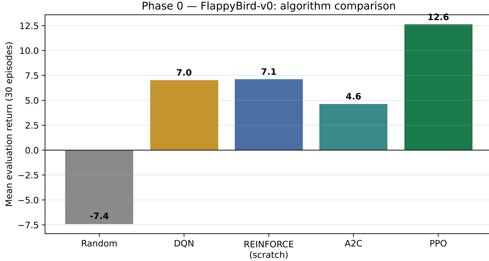
Figure 5.3: Flappy Bird comparison. PPO is the strongest learner under the fixed budget.
