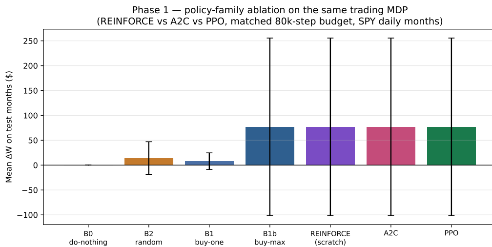
Figure 5.7: Policy-family ablation. REINFORCE, A2C and PPO execute the identical buy-max action sequence on every test month.
