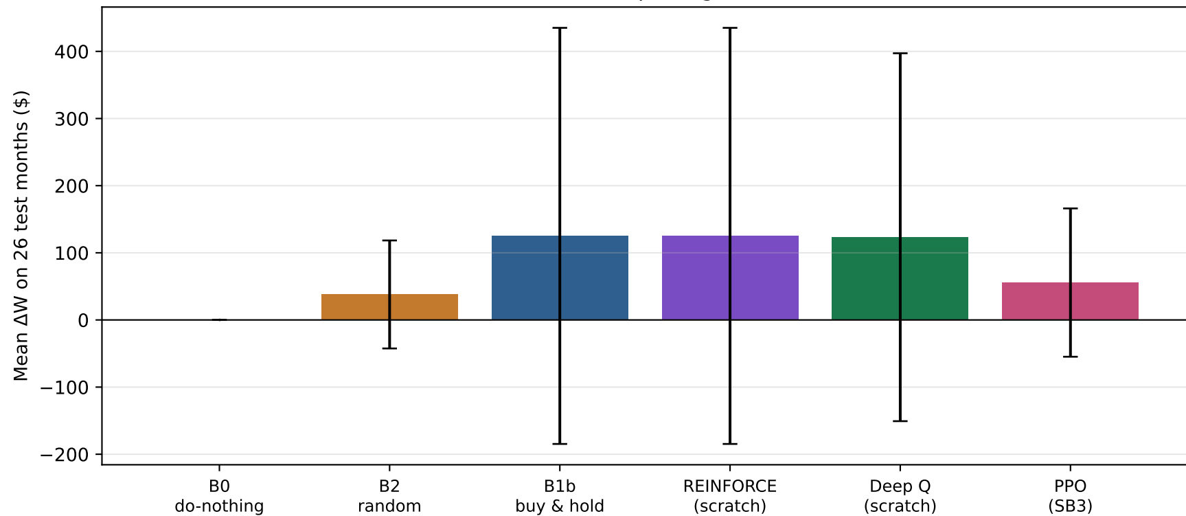
Algorithm ablation — complete 9-D state, divisible asset (matched 80k-step budget, seed 42)
