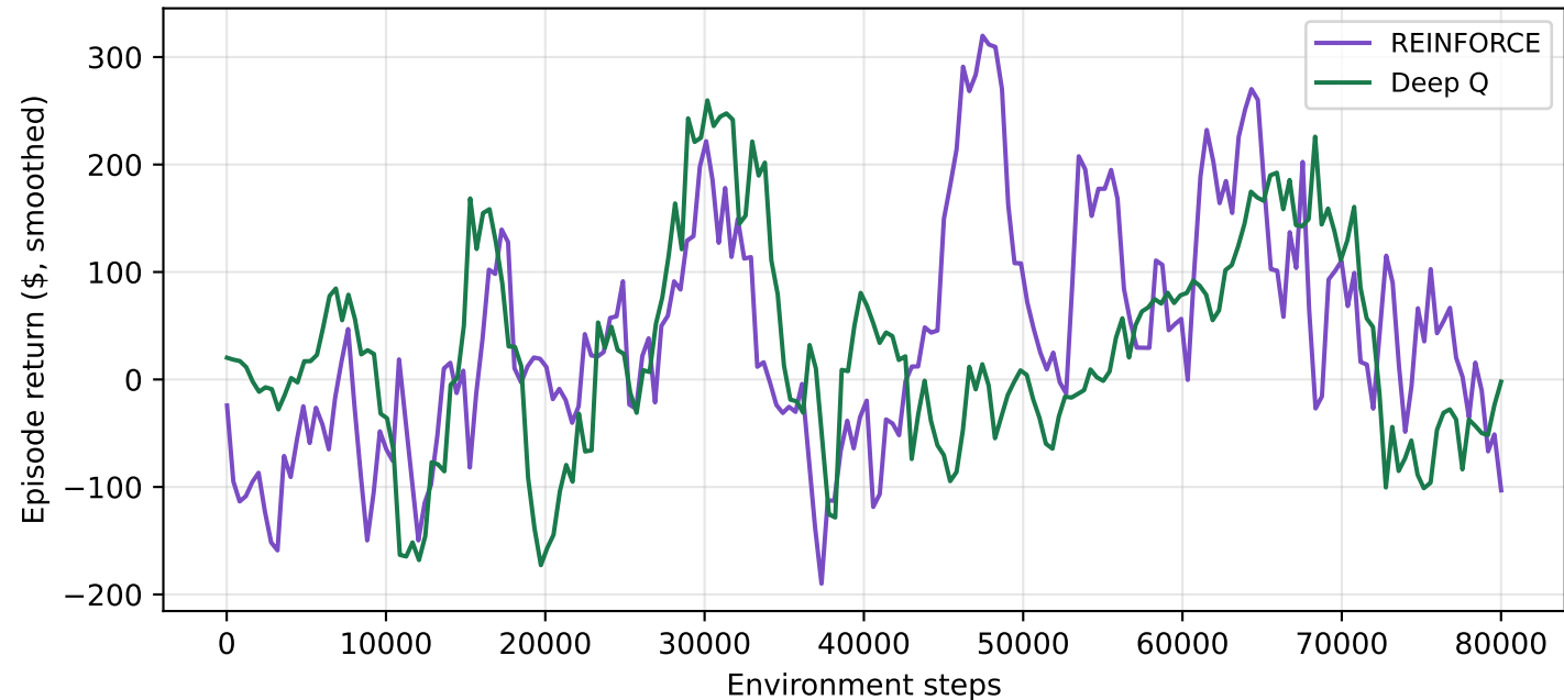
Training curves on the trading MDP (seed 42)
