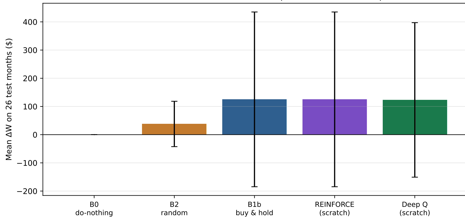
Final model — complete 9-D state, divisible asset (scratch REINFORCE vs scratch Deep Q, seed 42, 80k steps)
