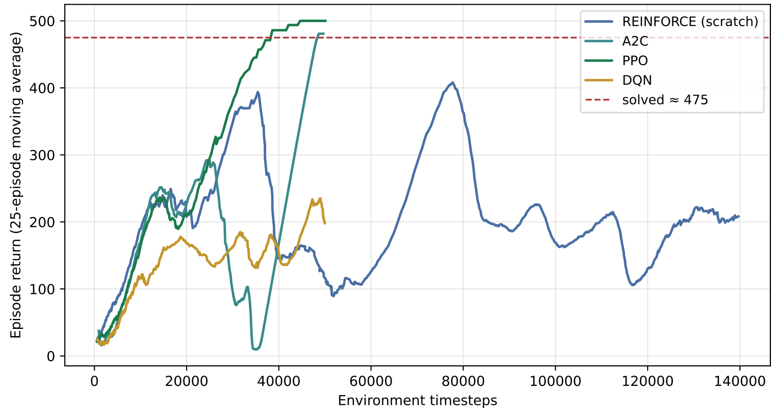
Phase 0 — CartPole-v1: learning curves
