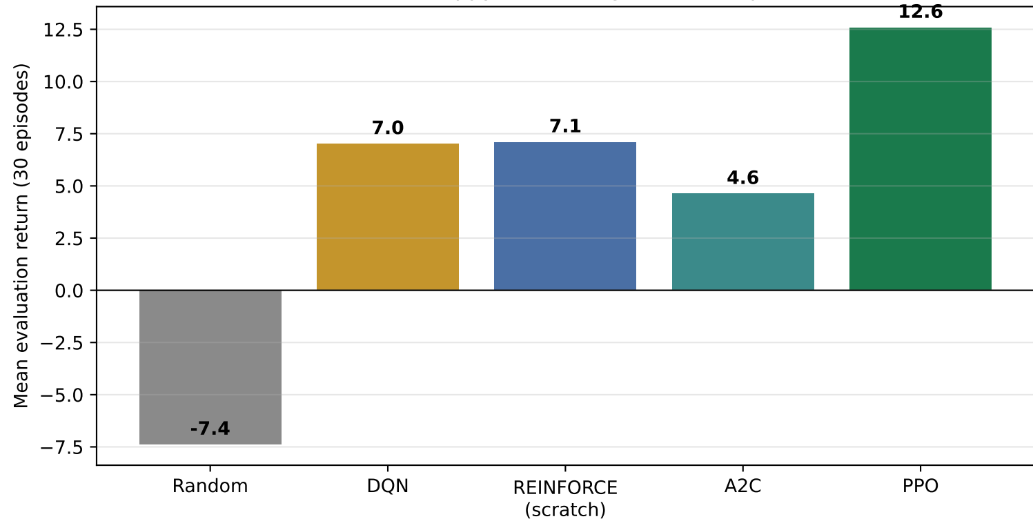
Phase 0 — FlappyBird-v0: algorithm comparison
