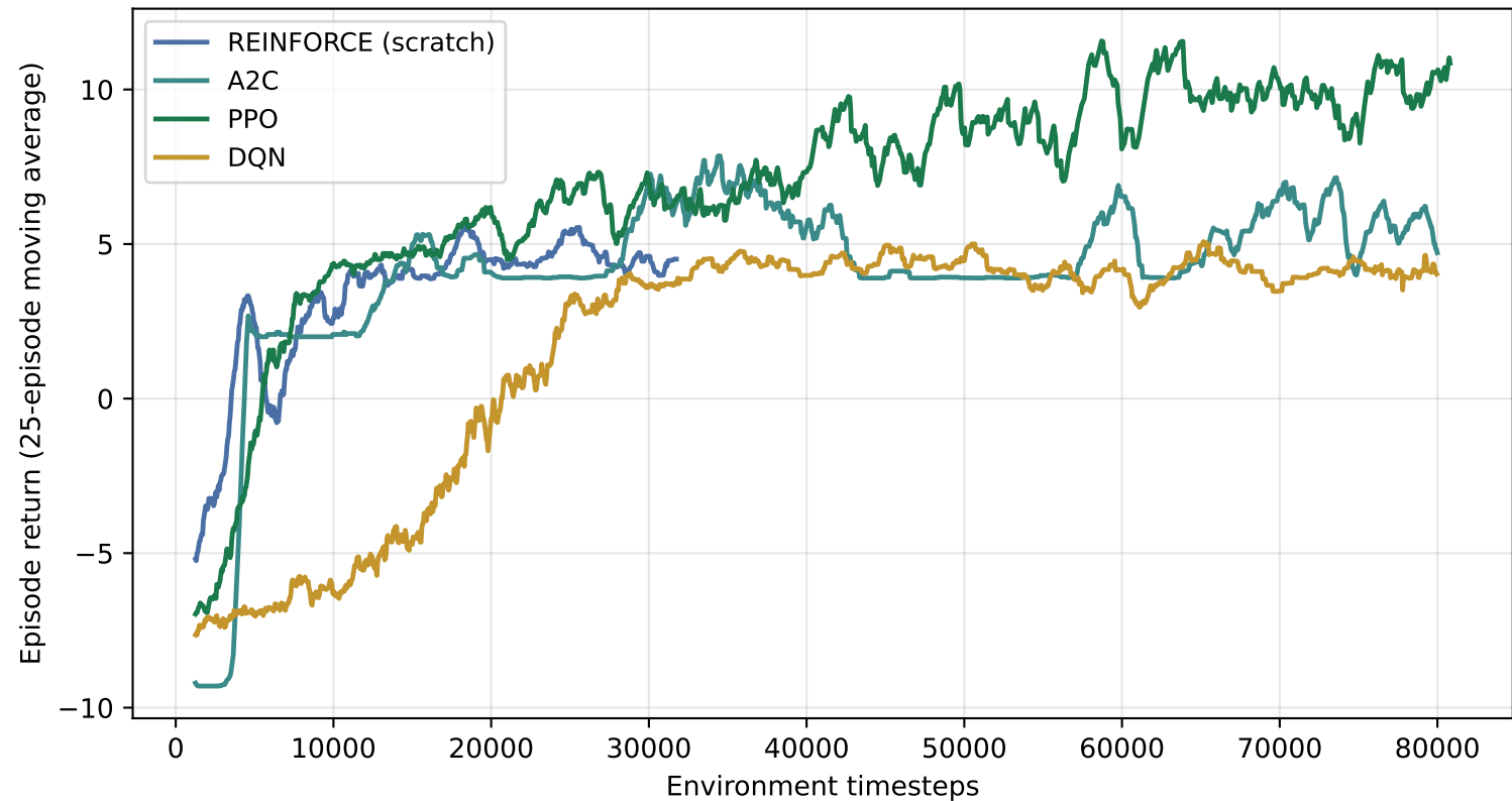
Phase 0 — FlappyBird-v0: learning curves
