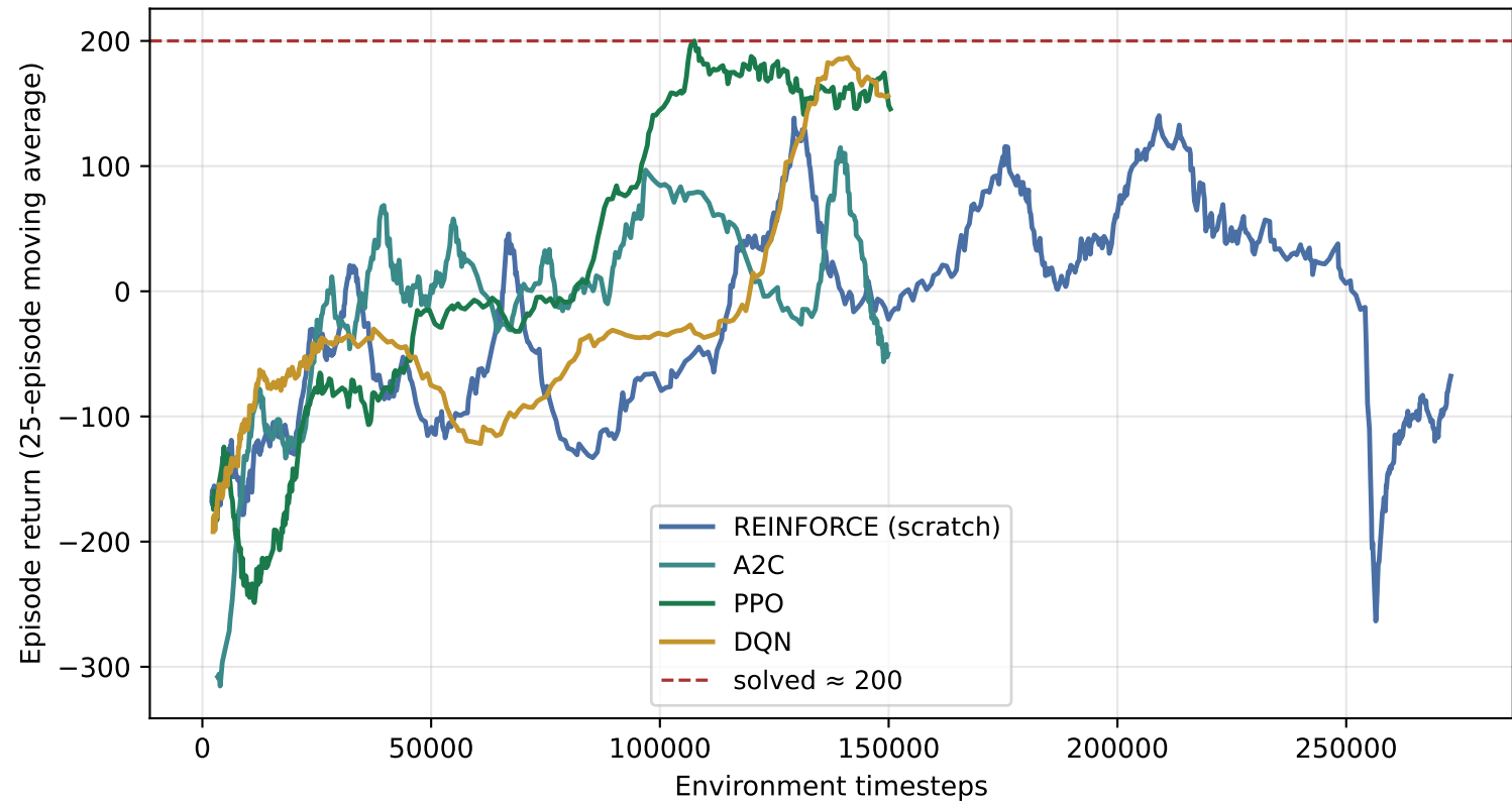
Phase 0 — LunarLander-v3: learning curves
