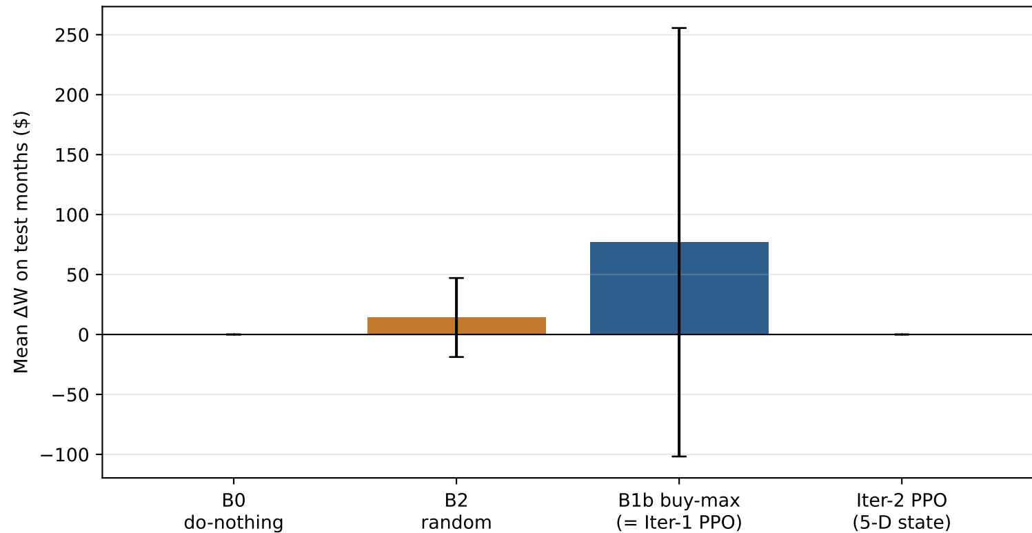
Phase 1 — Iteration 2 (5-D state) vs Iteration 1 on SPY test months
