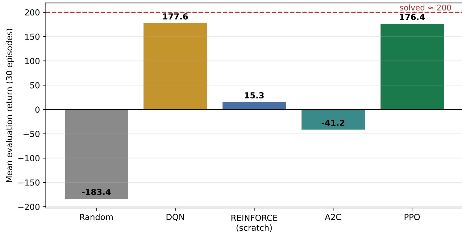
Phase 0 — LunarLander-v3: algorithm comparison
