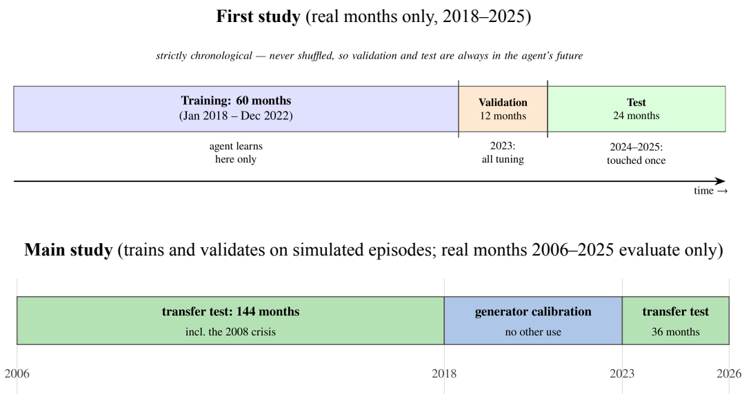
Figure 4.1: How the two studies use the real SPY months. The first study trains, validates, and tests inside 2018–2025 and never touches the earlier years. The main study reads real data only to calibrate the market generator (2018–2022); it trains and validates on simulated episodes, and every other real month — 2006–2017 and 2023–2025, 180 in total — becomes its transfer test.
