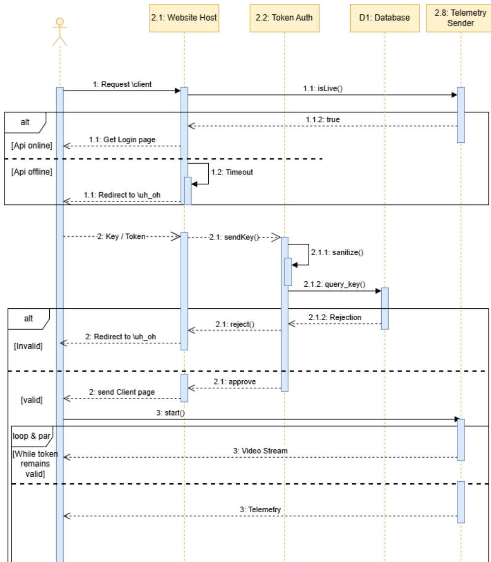
Figure 9: Sequence Diagram for User Connection to Web Client
