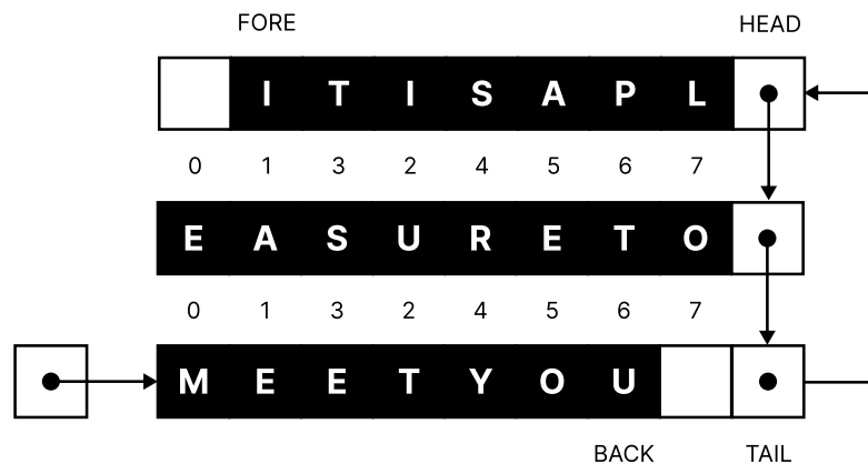
Figure 3.4: Graphical example of tail-based circular linked list of arrays. The front/fore element is the first element (index one) in the head node's array, and the back element is the last element (index six) in the tail node's array.
