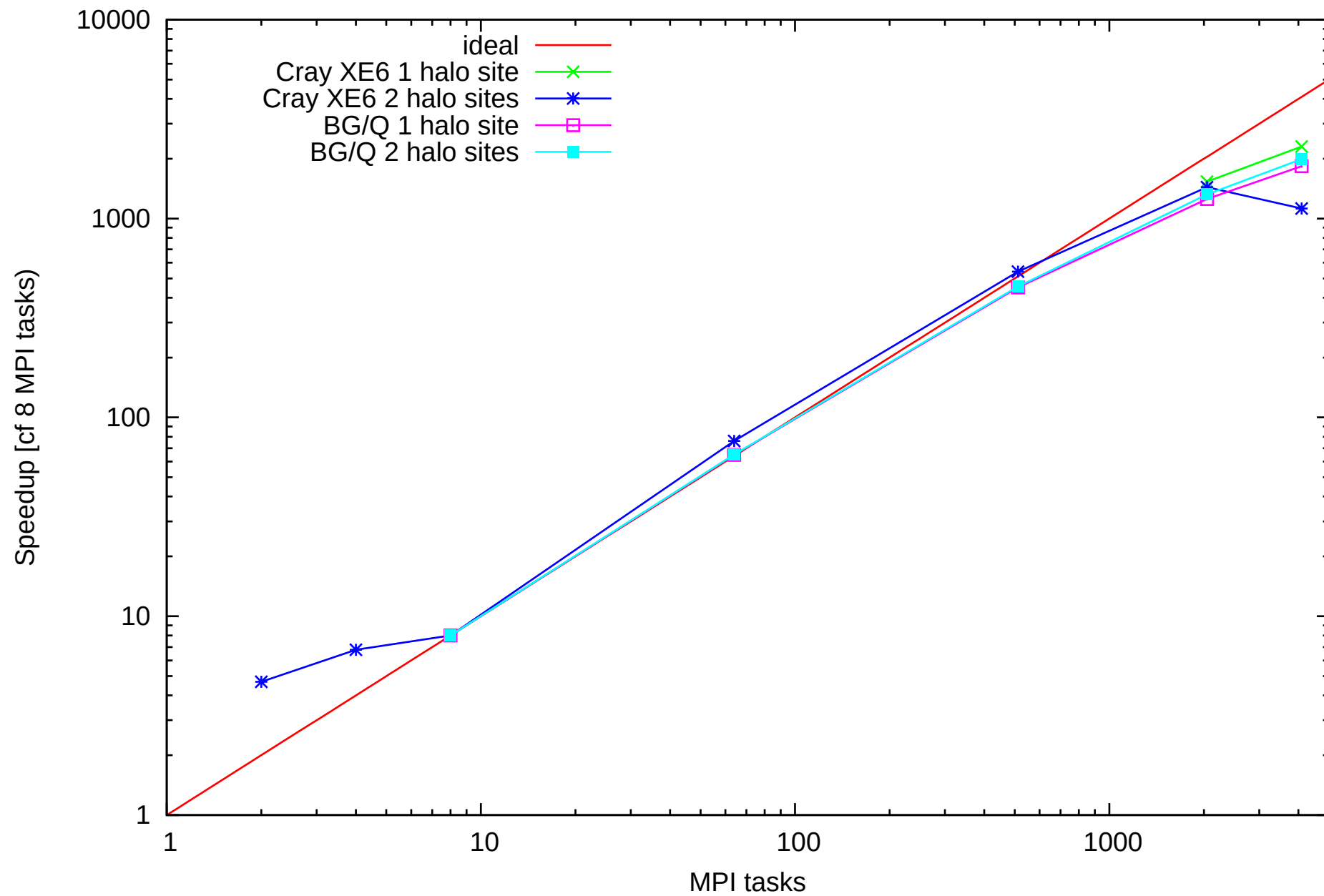
Ludwig Scaling: Poisson Solver + Nernst-Planck Equation, L=128^3
