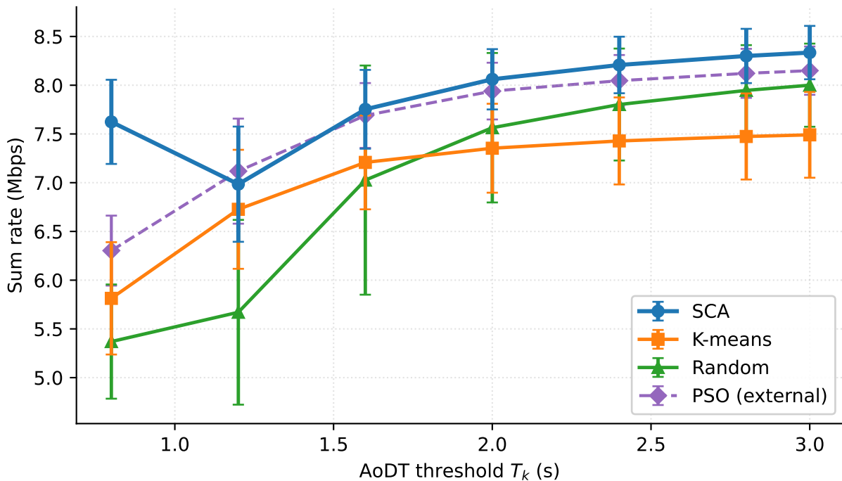
Fig. 9 analogue — sum rate vs AoDT threshold ( I = 10, J = 3 )
