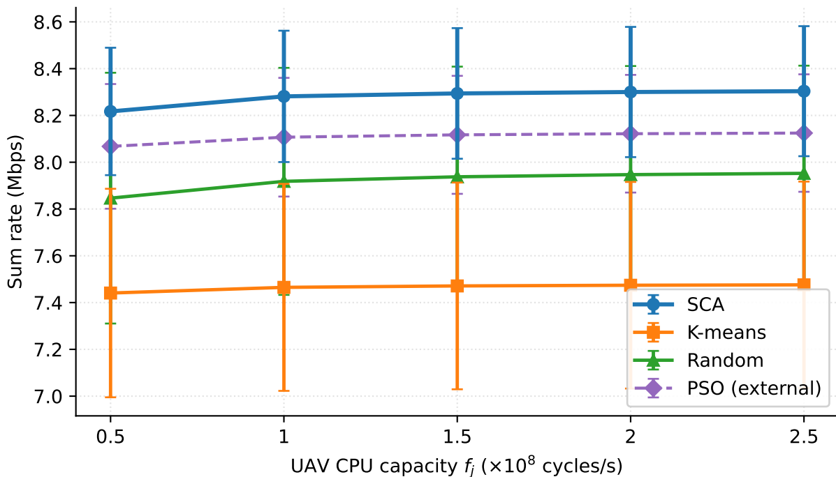
Fig. 10 analogue — sum rate vs UAV CPU ( I = 10, J = 3 )
