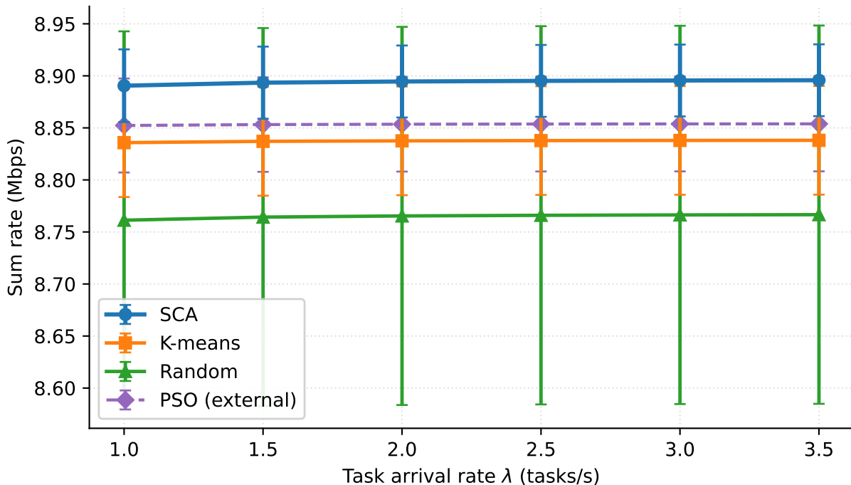
Fig. 8 analogue — sum rate vs arrival rate ( l = 10, j = 3 )
