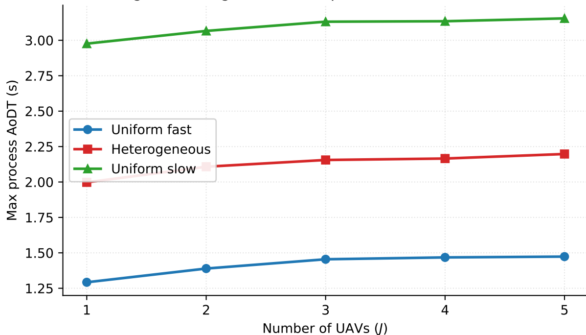
Fig. 11 analogue — arrival patterns (FCFS simulator)
