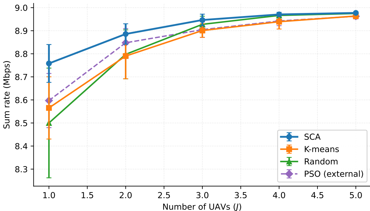
Fig. 6 analogue — sum rate vs UAV count ( l = 10 )
