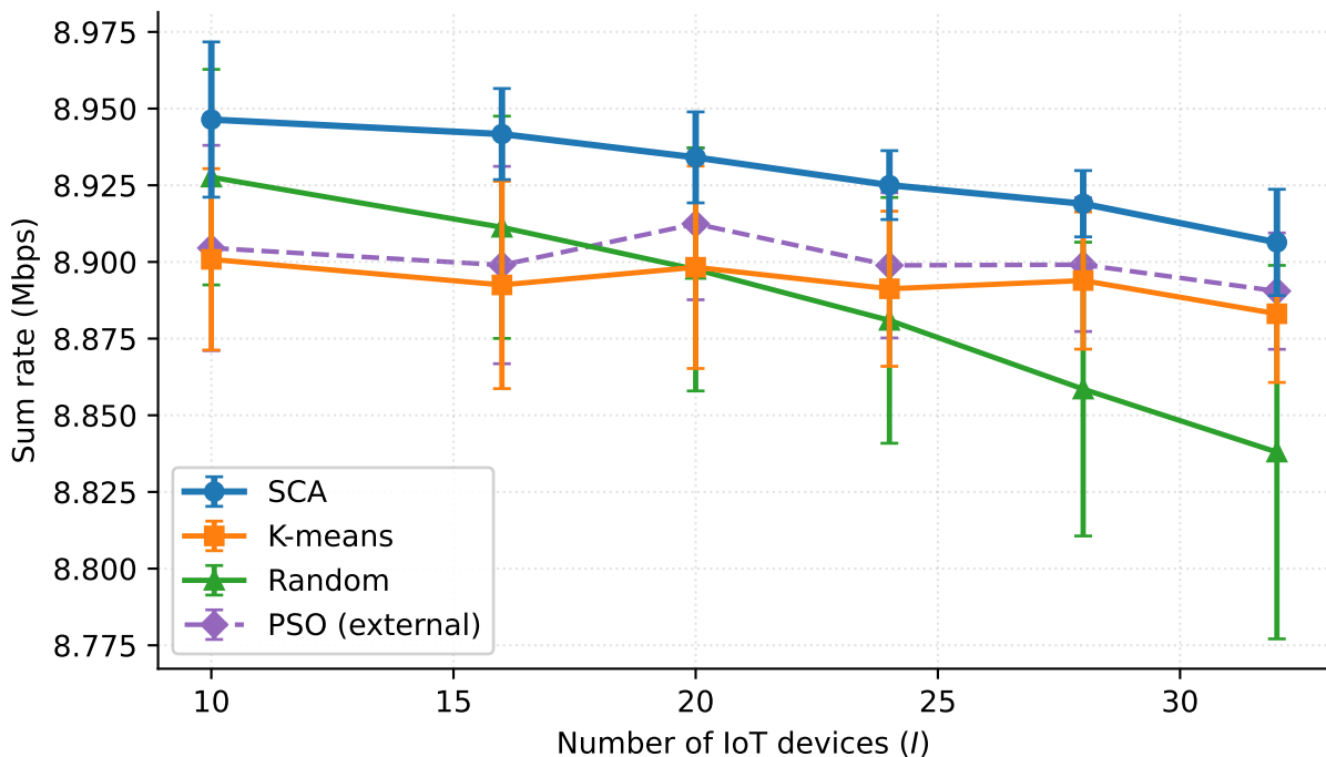
Fig. 7 analogue — sum rate vs IoT count ( J = 3 )
