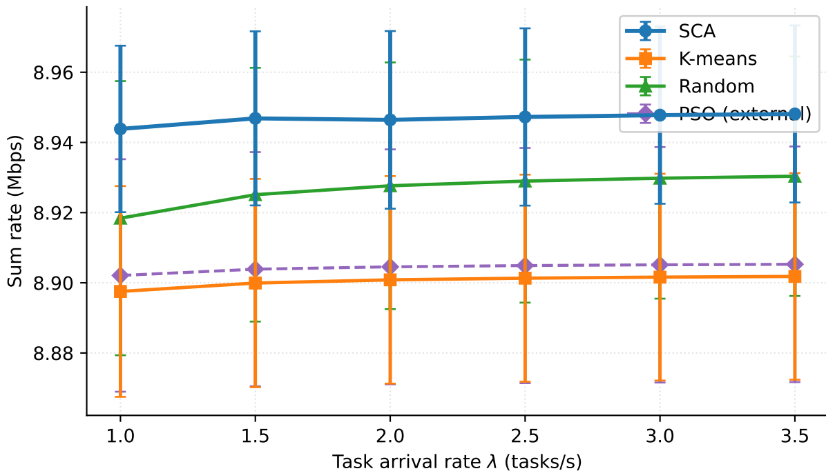
Fig. 8 analogue — sum rate vs arrival rate ( I = 10, J = 3 )
