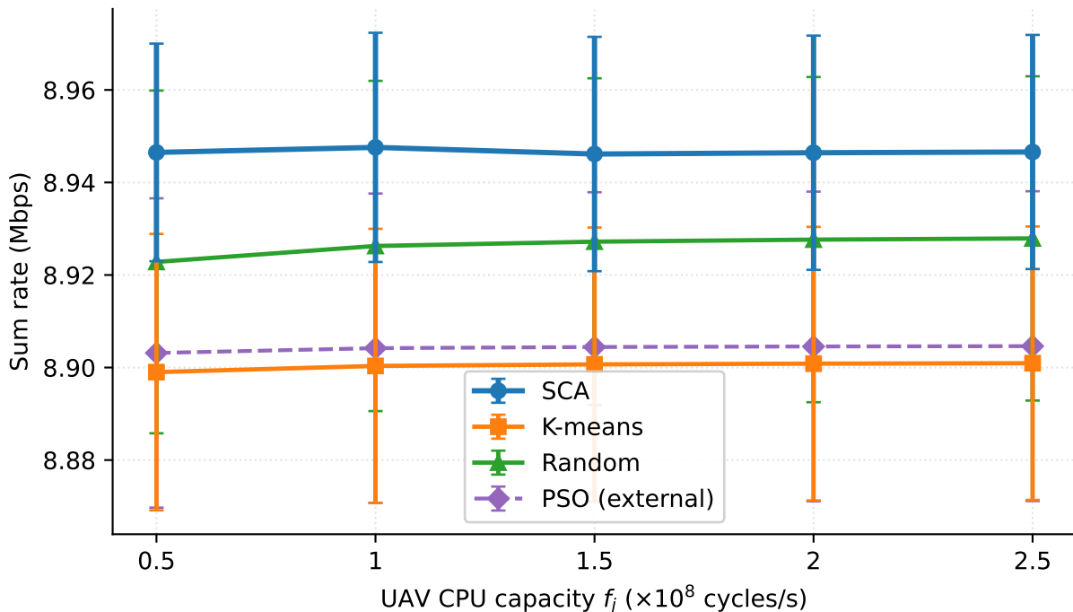
Fig. 10 analogue — sum rate vs UAV CPU ( l = 10, j = 3 )
