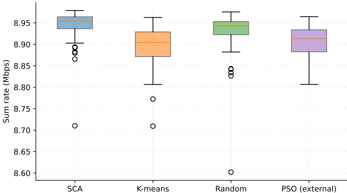
Per-scenario sum-rate distribution
