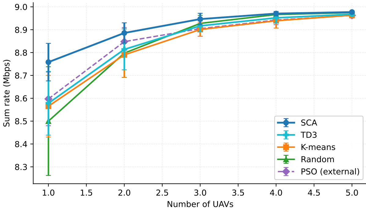
Sum rate vs UAV count
