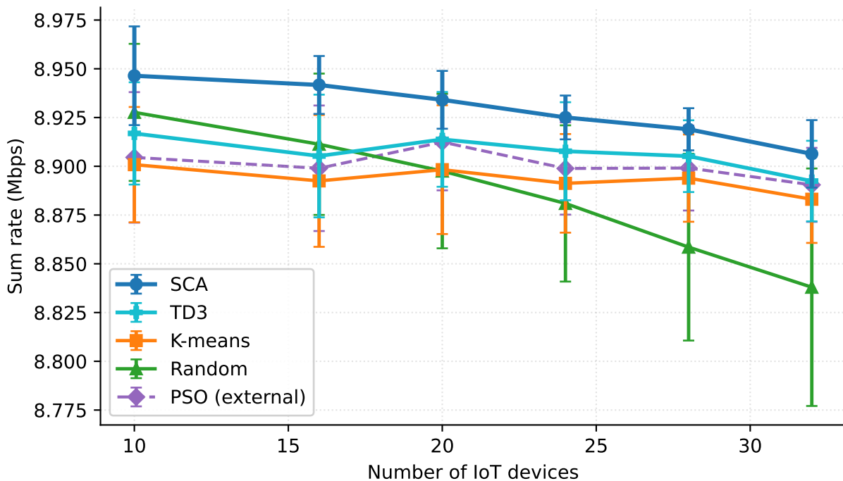
Sum rate vs IoT count
