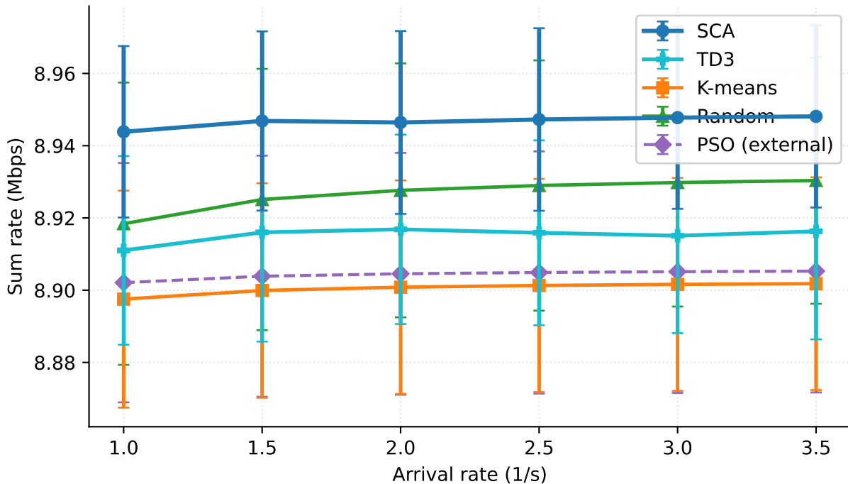
Sum rate vs arrival rate
