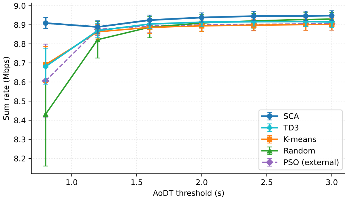
Sum rate vs AoDT threshold
