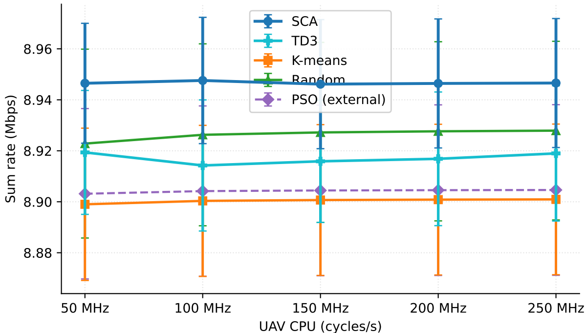
Sum rate vs computational capacity
