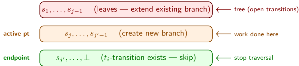
Figure 1.23: Partition of the boundary path into three zones when adding character t_i .
