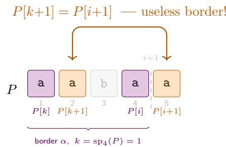
Figure 1.8: Strong border for P = \text{aabaa} at i = 4 . The border \alpha = \text{a} (violet, k = \text{sp}_4(P) = 1 ) satisfies P[1] = P[4] , but its “next character” P[k+1] = P[2] = \text{a} (orange) equals P[i+1] = P[5] = \text{a} . Any mismatch on P[5] with text character x \neq \text{a} would also fail immediately at P[k+1] after the fallback — the border is useless. Hence \text{sp}_4(P)' = 0 : skip straight to the start.
