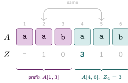
Figure 1.6: Z values for A = \text{aabaab} ( n = 6 ). The prefix A[1, 3] = \text{aab} (violet) reappears at position 4 (teal), giving Z_4 = 3 . Also Z_2 = Z_5 = 1 since A[1] = A[2] = A[5] = \text{a} , and Z_3 = Z_6 = 0 since A[3] = A[6] = \text{b} \neq A[1] . Z_1 is left undefined.
