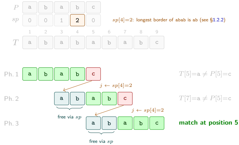
Figure 1.6: KMP search for P=\text{ababc} ( m=5 ) in T=\text{ababababc} ( n=9 ). The sp array for P is shown at the top (cf. the preprocessing in §1.2.2). Green: characters newly matched in this phase. Teal: characters carried for free from the previous phase via j \leftarrow sp[j] . Red: mismatch. After each fallback, the algorithm reuses the last sp[j] matched characters without any comparison, then continues from where it left off in T .
