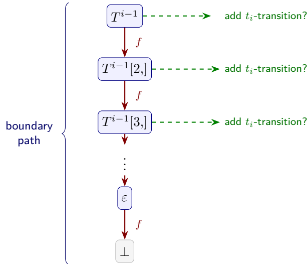
Figure 1.21: The boundary path of \text{STrie}(T^{i-1}) : the chain of suffix links from the deepest state T^{i-1} down to \perp . To build \text{STrie}(T^i) we walk this path and add a t_i -transition from every state that does not already have one.
