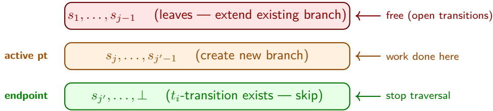
Figure 1.22: Partition of the boundary path into three zones when adding character t_i .
