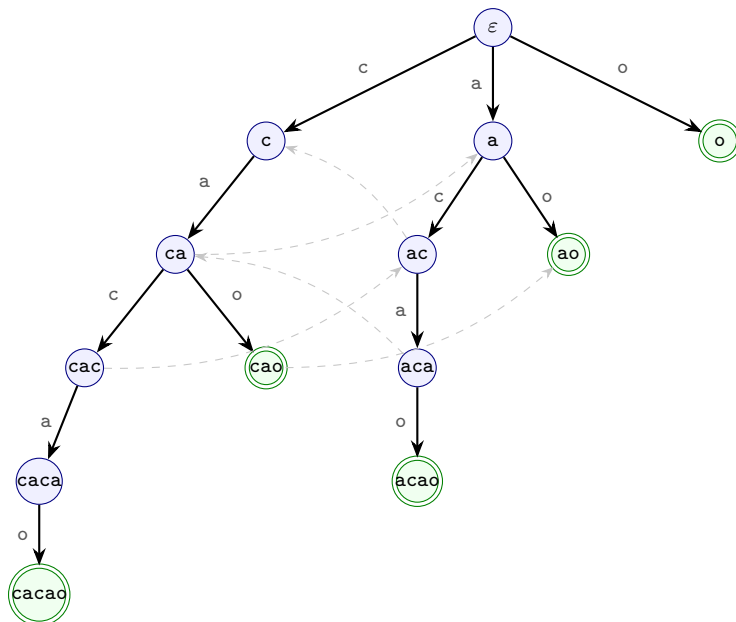
Figure 1.19: Suffix trie \text{STrie}(\text{cacao}) . Solid arrows are transitions g'(s, a) ; dashed arrows show selected suffix links f(s) . Double-bordered states are final (they correspond to actual suffixes). Every path from the root spells a distinct substring of \text{cacao} .
