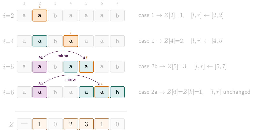
Figure 1.7: Z-box algorithm on A = \text{aabaaab} (steps i=3 and i=7 omitted: Z=0 , no update). Teal : current Z-box [l, r] . Orange border : current position i (filled teal when i is inside the box). Violet : mirror k = i - l + 1 , with arc showing the mirror correspondence. Bottom row: final Z array (non-zero entries highlighted).
