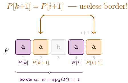
Figure 1.9: Strong border for P = \text{aabaa} at i = 4 . The border \alpha = \text{a} (violet, k = \text{sp}_4(P) = 1 ) satisfies P[1] = P[4] , but its “next character” P[k+1] = P[2] = \text{a} (orange) equals P[i+1] = P[5] = \text{a} . Any mismatch on P[5] with text character x \neq \text{a} would also fail immediately at P[k+1] after the fallback — the border is useless. Hence \text{sp}_4(P)' = 0 : skip straight to the start.
