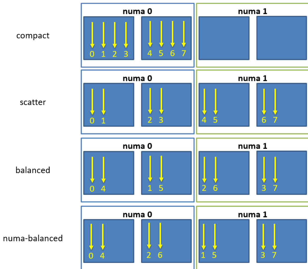
Fig. 2.7: Schematic of thread affinity type distributions.
