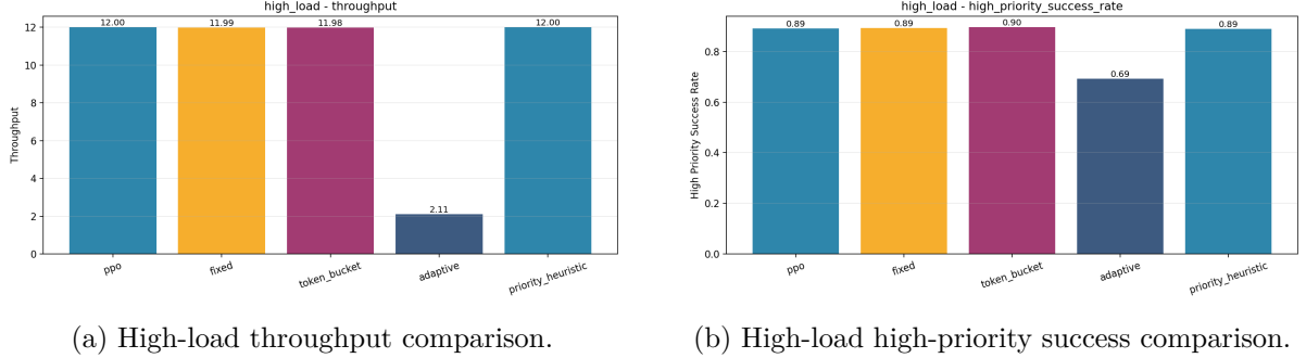
Figure 3: Count-based high-load plots from the final evaluation pipeline. These emphasize that PPO can be highly competitive once the high-priority penalty is no longer overly conservative.
