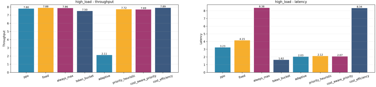
(a) High-load throughput across PPO and heuristics.
