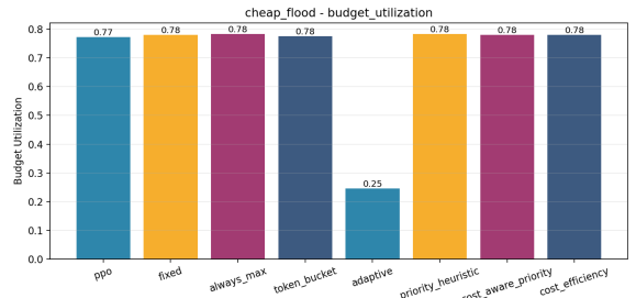
(b) Cheap-flood budget utilization.
