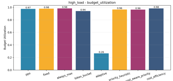
(b) High-load budget utilization.
