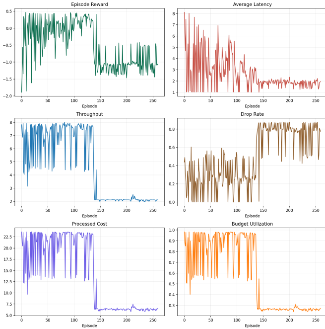
Fig. 4: Training curves for the naive cost-aware PPO. After a promising mid-training phase, reward and throughput collapse while the agent drifts toward a near-always-decrease policy.
