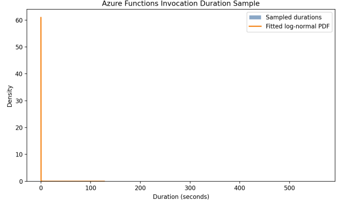
Fig. 9: Histogram of sampled Azure Functions invocation durations with a fitted log-normal density overlay. The raw duration distribution is extremely heavy-tailed, motivating the separate Azure-calibrated transfer test for cost-aware policies.
