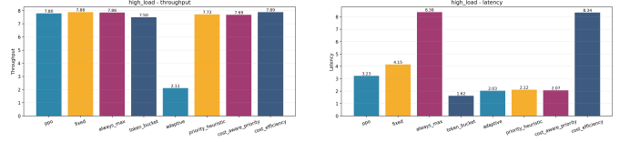
(a) High-load throughput across PPO and heuristics. (b) High-load latency across PPO and heuristics.
