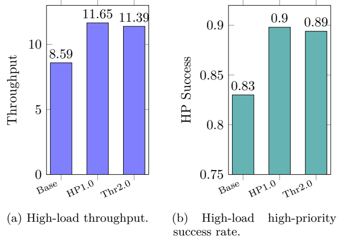
Fig. 1: Count-based reward ablation on the high-load scenario. Lowering the high-priority penalty fixes the over-conservative regime; increasing throughput weight maximizes scalar reward but produces a different trade-off.
