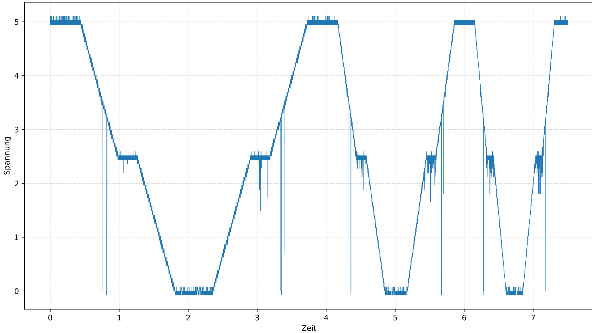
Rauschkurve Test01_DS_10
