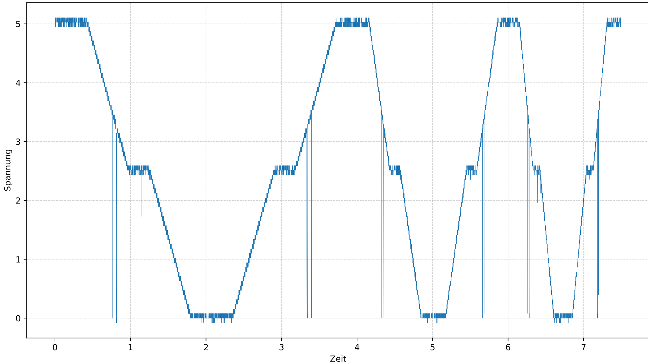
Rauschkurve Test03_DS_25
