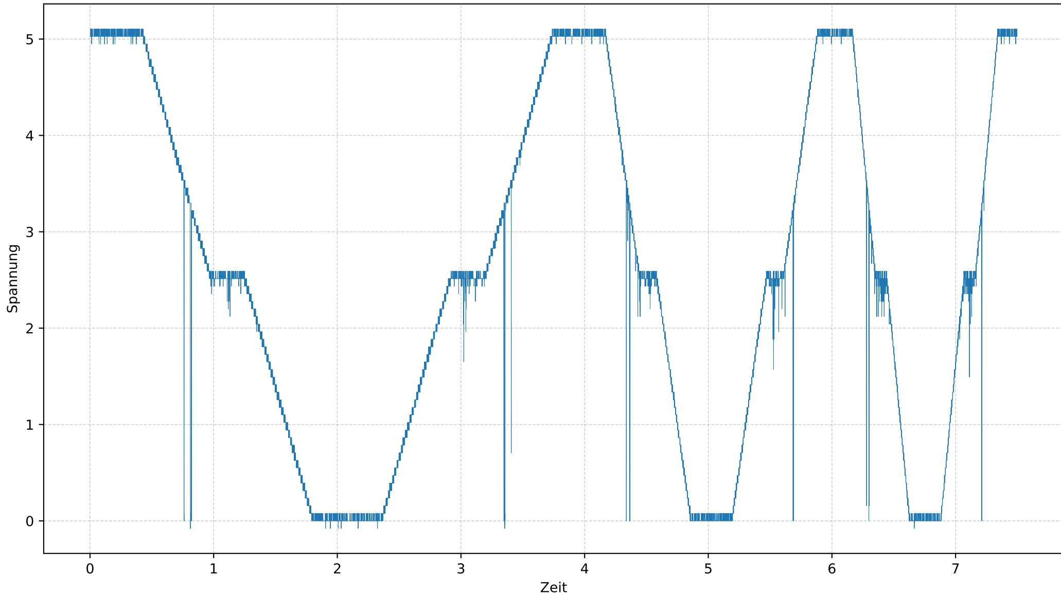
Rauschkurve Test04_DS_50
