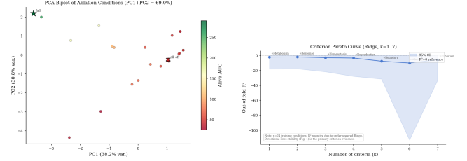
Figure 10: Left: PCA biplot (PC1=38%, PC2=31%; full-criteria vs. all-off at opposite poles; pairwise ablations cluster near all-off). Right: criterion Pareto curve (all R^2 < 0 ; underpowered; Enet rankings are primary evidence).
