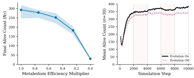
Figure 21: Left: graded metabolic ablation dose-response (median \pm IQR, n=30 per level; p < 0.001 , Jonckheere-Terpstra). Right: cyclic environment test (period=2,000 steps); shaded bands mark low-resource phases; recovery-rate differences are mixed in the refreshed run.
