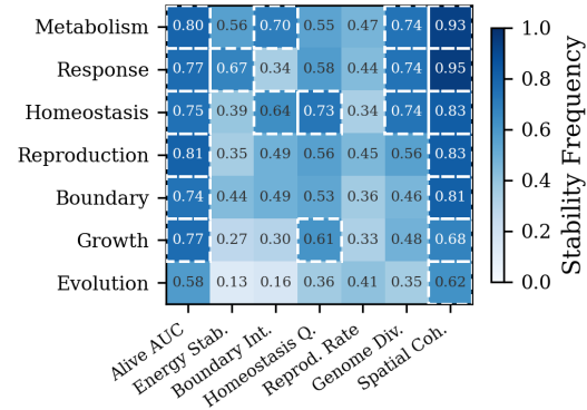
Enet Stability Heatmap: Criterion \times Performance Metric
