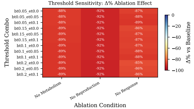
Figure 19: Threshold sensitivity heatmap: \Delta\% ablation effect for each threshold combination \times ablation condition. Rank ordering of effects is assessed via Spearman correlation with the default-threshold ranking.
